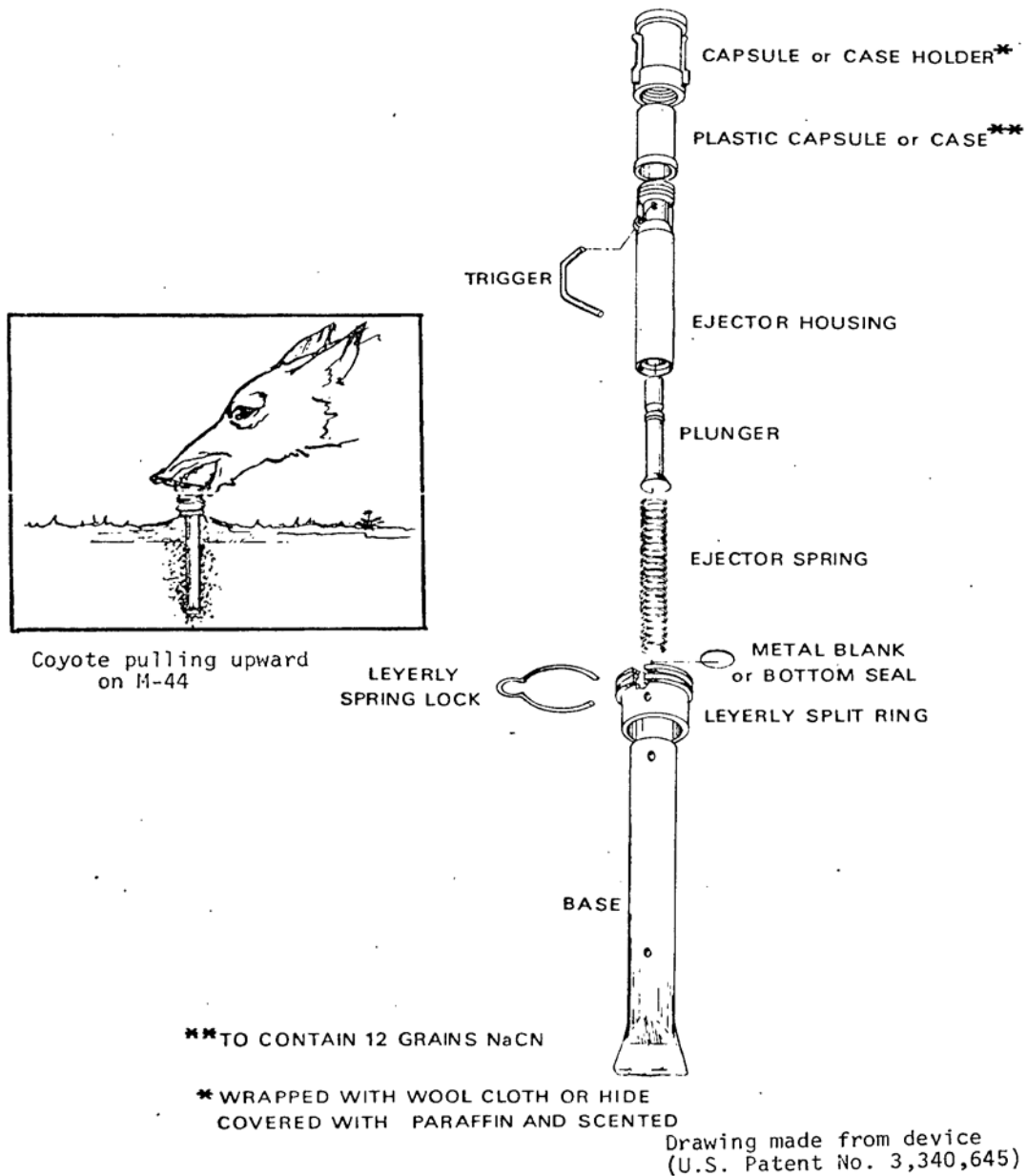
Figure 1. M-44 Components
